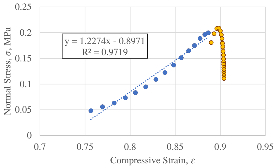
Figure C 8. Normal stress, \sigma , versus compressive strain, \epsilon , for dynamic EA (80 RPM) tissue segment 18b.
