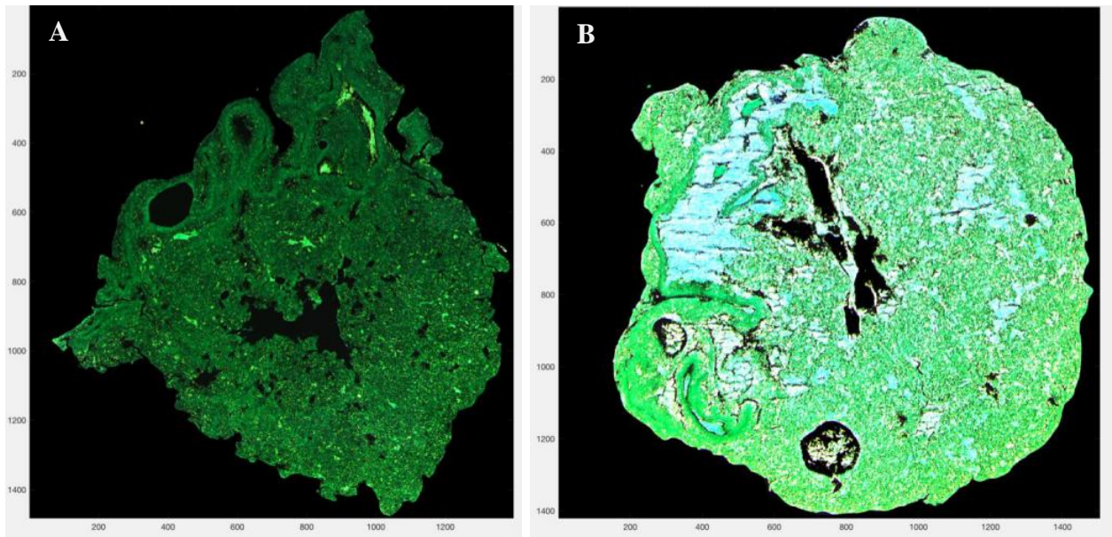
Figure 7. Optical density (OD) images of tissue sections from (A) EA formed at 80 RPM and (B) EA formed at 34 RPM. Axes indicate image dimensions in pixels.
